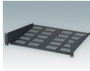
M6119284 19"x2U Cantilever Rack Shelf Mild Steel CR4 Anthracite RAL 7016 88.1x482.6x400mm
