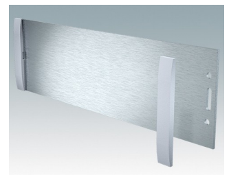
M5700613 Front panel kit (3/3H) Aluminium Matt anodised 219.5x2x65.1mm
