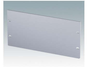
M6010001 Front panel 3Ux10.5" Aluminium Matt anodised 269.2x3x132.5mm
