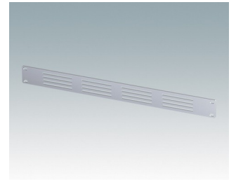
M6019011 Front panel 1Ux19" vented Aluminium Matt anodised 482.6x3x43.6mm
